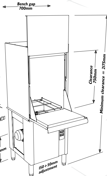
Wash Chamber
